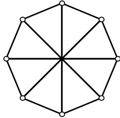
Figure 6.1: The graph V_8 .
