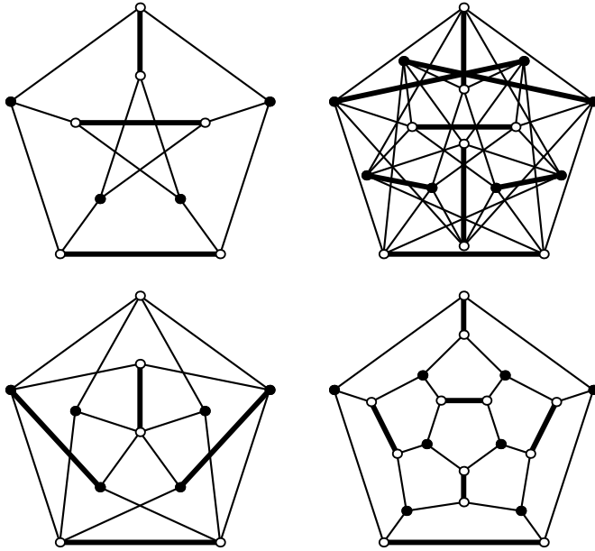
Figure 1.2: Examples of graphs that are TT_2 -equivalent to C_5 : Petersen graph, Clebsch graph, Grötsch graph, and graph of the dodecahedron. One color class is emphasized, the respective bipartition of the vertex set is depicted, too. The other four color classes are obtained by a rotation.
