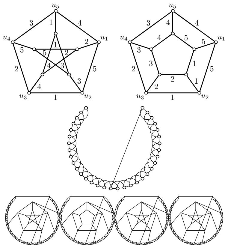
Figure 2.2: Petersen graph, P_t , and the prism R of C_5 —two TT_2 -equivalent graphs used in the proof of Proposition 2.1.10. Below is a graph that we use as a ‘frame’ to hold one of the two graphs above, and an example of the construction for n = 4, t = (1, 0, 1, 1) .
