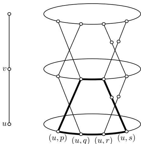
Figure 3.4: Example of construction of F(G) for G = P_2 . The 7-cycle used in the proof of Theorem 3.2.2 is emphasized.
