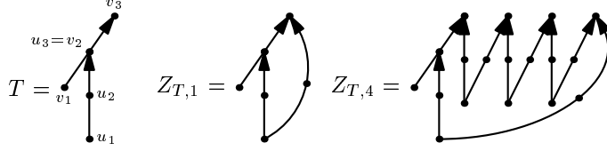
Fig. 1. An example of thunderbolts for structures with a ternary relation
