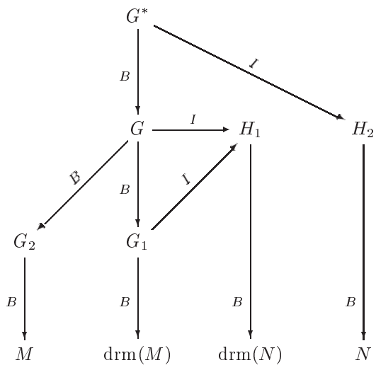
Figure 6: Commutative diagram for the proof of Proposition 35.
