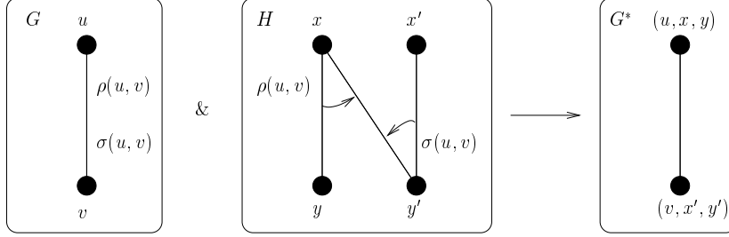
Figure 8: Construction of the graph G^* .
