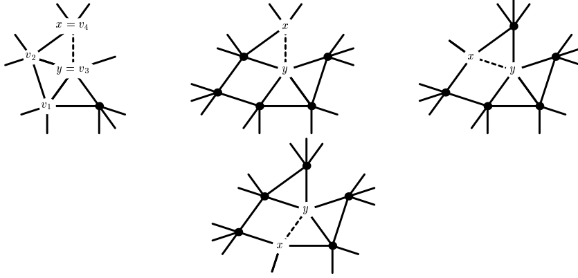
Figure 11: The degree configurations from Lemma 5.6.
