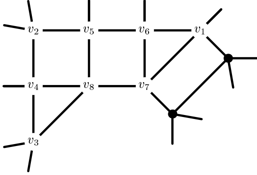
Figure 22: The degree configuration from Lemma 6.12.
