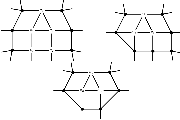
Figure 17: The degree configurations from the proof of Lemma 6.8.
