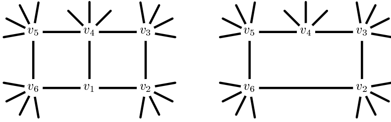
Figure 3: The configuration from Lemma 4.3 and its replacement.
