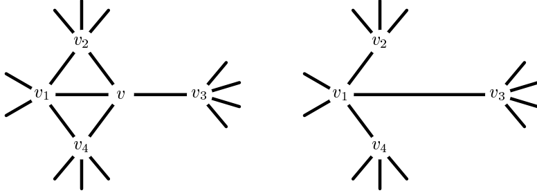
Figure 10: The configuration from Lemma 5.5 and its reduction.
