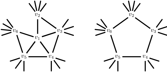
Figure 6: The configuration from the Lemma 4.6 and its replacement.
