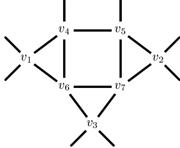
Figure 19: The degree configuration from the proof of Lemma 6.9.
