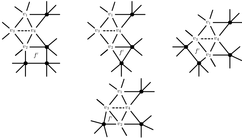
Figure 12: The degree configurations from Lemma 5.8.
