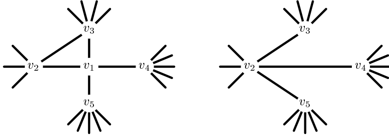
Figure 5: The configuration from Lemma 4.5 and its replacement.
