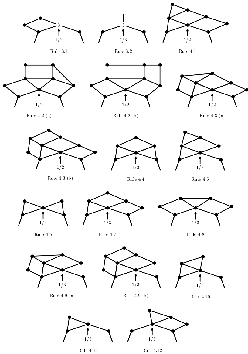
Figure 25: Rules 3.1–4.12 used in Section 6.
