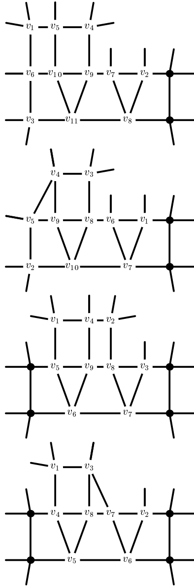
Figure 24: The degree configurations from Lemma 6.14.
