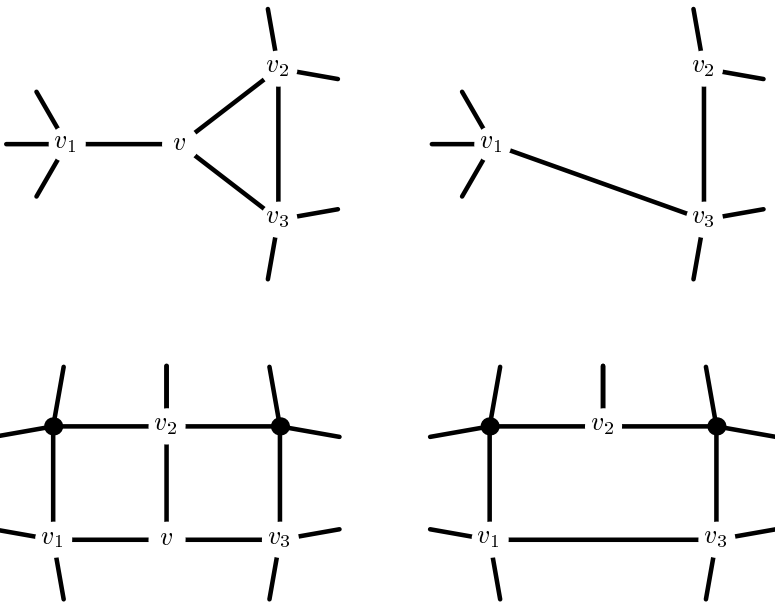
Figure 14: The configurations from Lemma 6.5 and their reductions.
