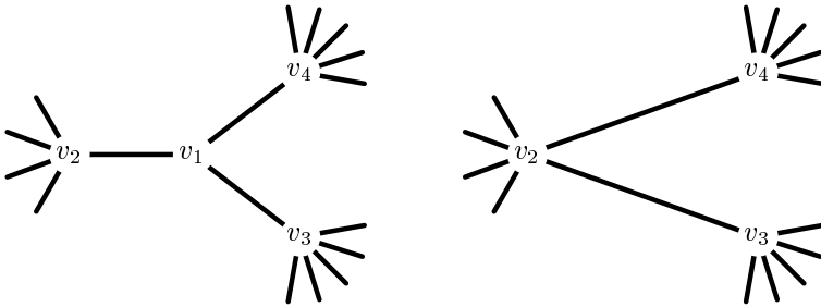
Figure 4: The configuration from Lemma 4.4 and its replacement.
