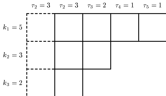
Figure 3: The conjugation of the sequences k_1, \dots, k_r and \tau_1, \tau_2, \dots, \tau_\ell from the example in Figure 2.
