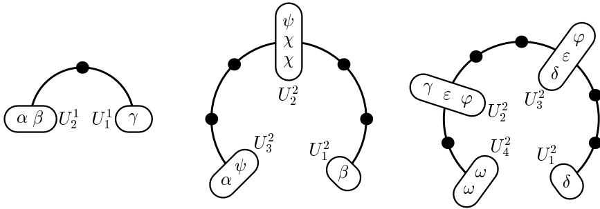
(ii) partitioning V_c into sets U_j^i
