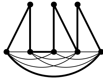
(iv) a Hamilton cycle
