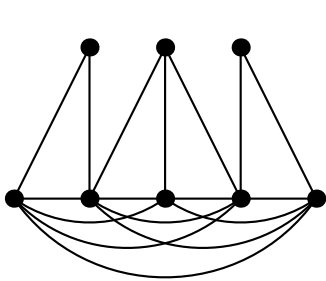
(i) a graph G
