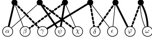
(i) the auxiliary graph H
