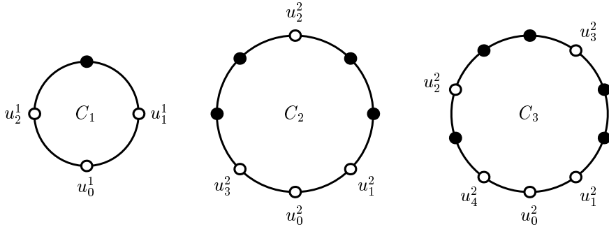
(i) Hamilton cycles in graphs G'_1 , G'_2 and G'_3
