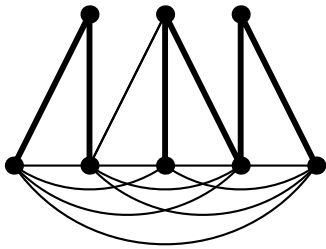
(iii) a subgraph G''
