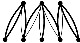
(ii) the graph G^* and a subgraph G' the edges of the clique of G^* are omitted
