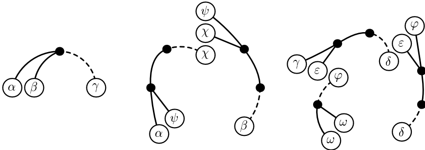
(iii) the collection of paths (red edges are dashed)
