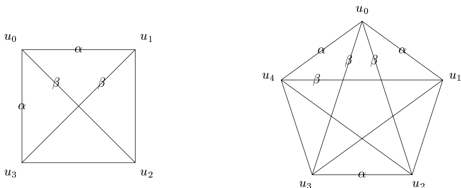
FIGURE 3. Proving Proposition 4.4.
