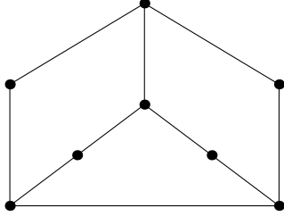
Figure 3: A 5-minimal graph
