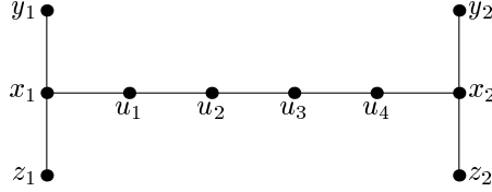
Figure 4: The graph H_4 .
