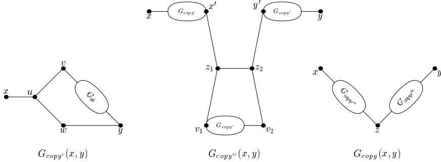
Figure 7: Graphs used in Lemma 24
