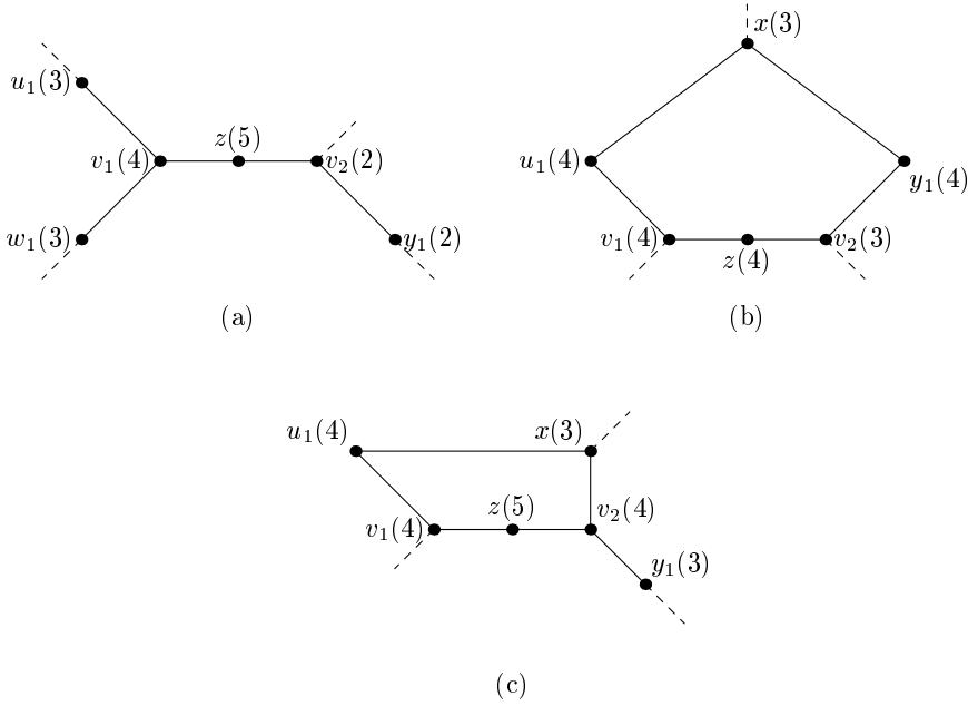
Figure 2: Configurations arising from Y_{1,1}-1-Y_{0,1}
