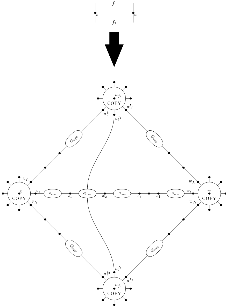
Figure 9: The NP-completeness reduction
