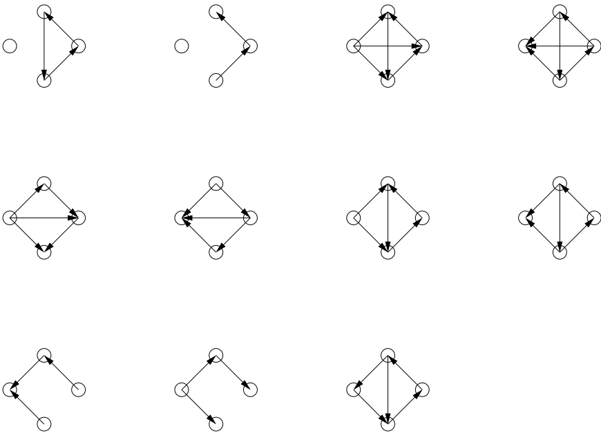
Fig. 3. The forbidden induced subgraphs of P(3) .
