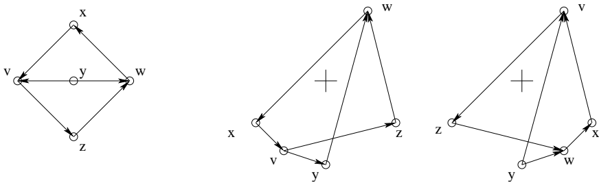
Fig. 2. On the left we find the gadget to simulate with \text{CSP}(S(2)) the betweenness relation on x, y, z , where an arc from a to b means that there is the constraint a < b . On the right we find two possible ways to map these vertices homomorphically to S(2) , where the cross marks the origin in the plane.
