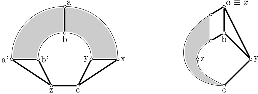
Figure 3: Configurations in Lemma 8
