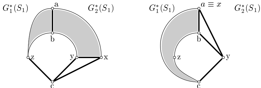
Figure 2: Configurations in Lemma 7
