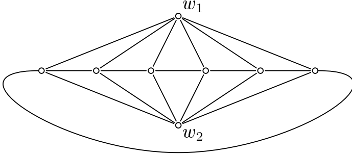
Figure 1: A double wheel
