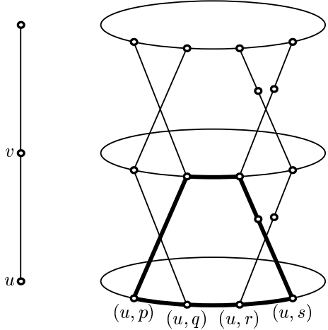
Fig. 5 Example of construction of F(G) for G = P_2 . The 7-cycle used in the proof of Theorem 12 is drawn bold.
