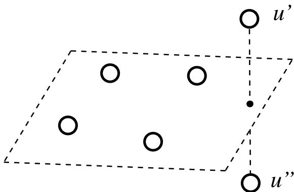
Figure 5. Blowing a vertex of the pentagon.
