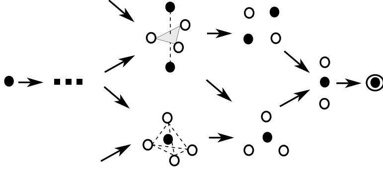
Figure 4. The interval K_1 \rightarrow K_2 in \mathcal{P} .
