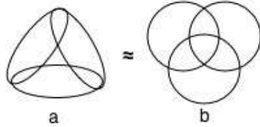
Figure 1. Two representations of K_3 in \mathbb{E}^2 .
