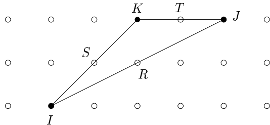
Figure 1: The points R, S, T .
