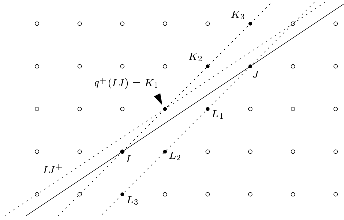
Figure 4: The lattice points K_i, L_i .
