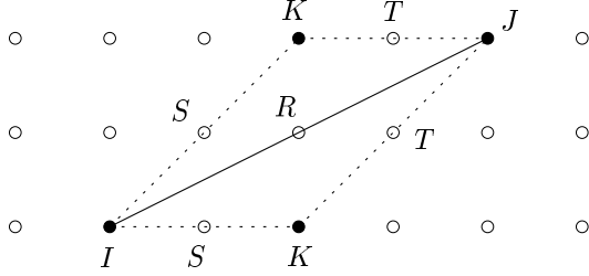
Figure 2: Two possible placements of K .
