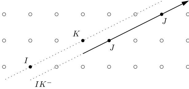
Figure 3: The lattice points J with K = q^+(IJ) .
