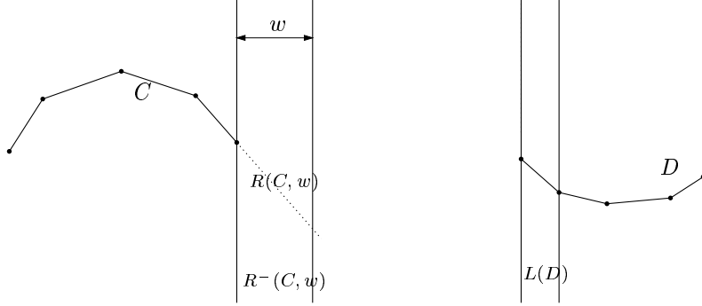
Figure 3: The regions R(C, w) , R^-(C, w) and L(D) .
