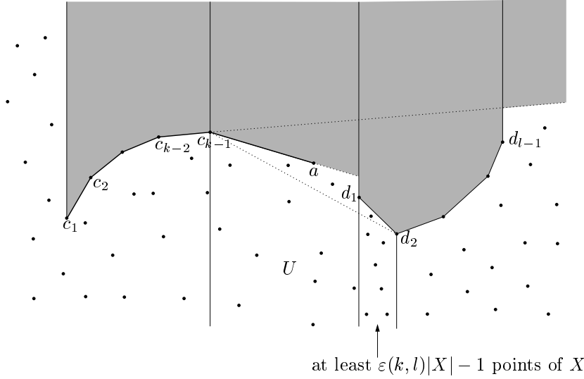
Figure 8: Case 1 (the shaded regions contain no points of X ).
