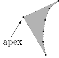
Figure 2: A 7-moon; it is empty in X if the shaded region contains no points of X .
