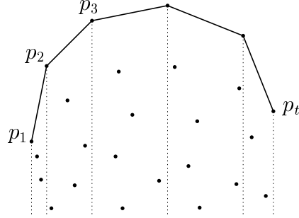
Figure 7: The upper envelope of X .
