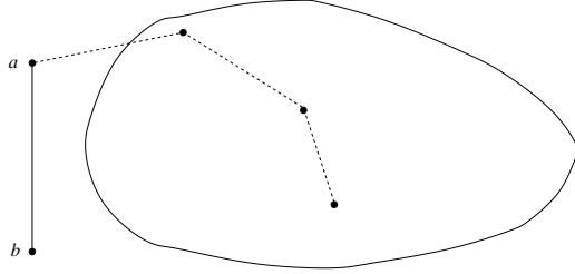
Figure 3: A vertical point set with a 5-cap.
