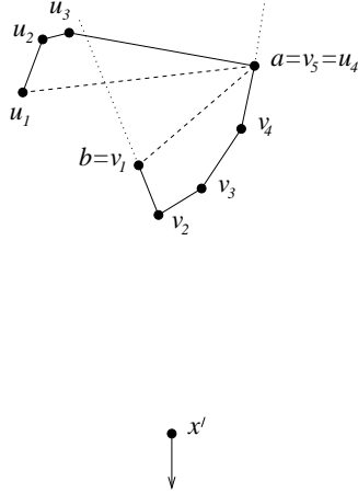
Figure 5: x', u_1, u_2, u_3, v_1, v_2 determine a convex hexagon.
