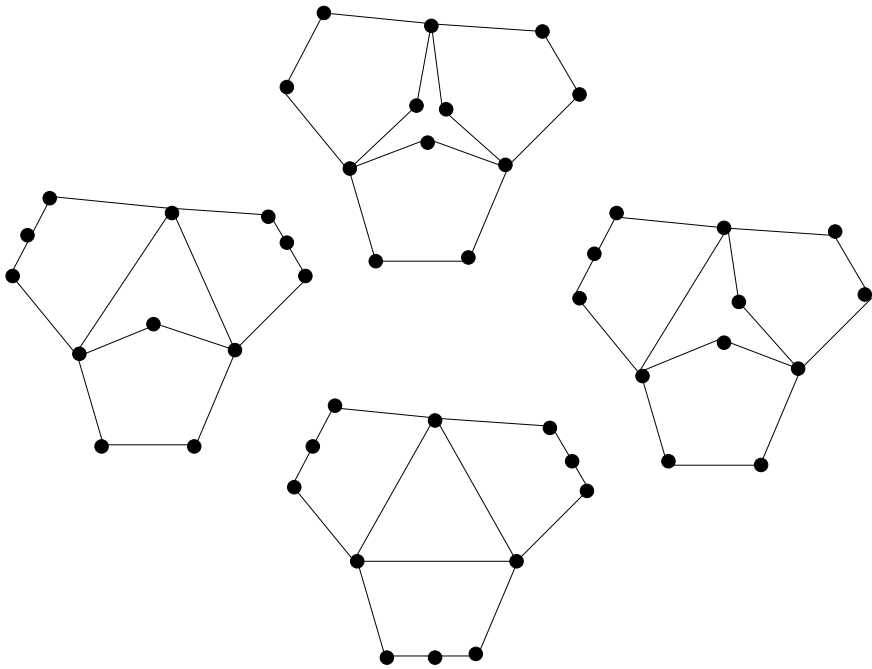
Figure 4: Only the 3-Pentagon is without K_2 -separation
