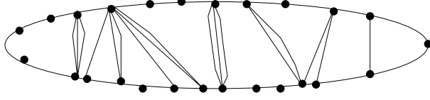
Figure 2: A Hamiltonian Outer-planar graph is a ladder
