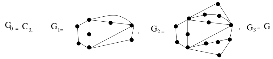
Figure 7: An example of construction by recursion
