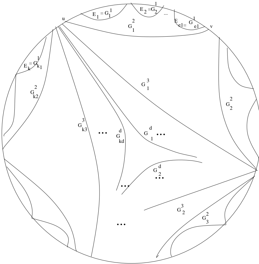
Figure 6: A general structure of a 2-connected graph in SPG
