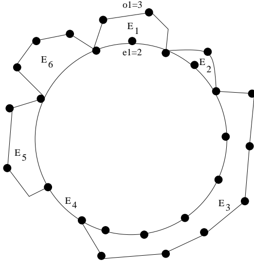
Figure 5: A 6-ear-face with five ears and one diminished-ear
