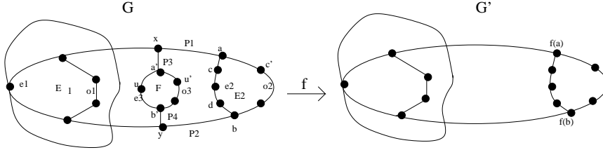
Figure 3: A homomorphism from G to G' contradicts the choice of G
