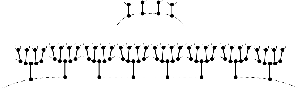
Figure 1: Examples of octopuses for p = 2 and p = 4 .
