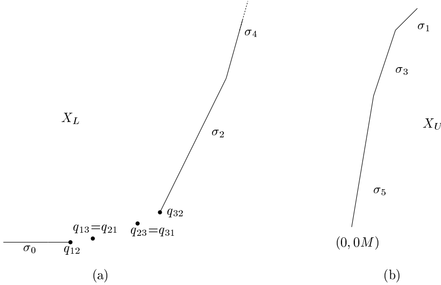
Figure 2: (a) The set X_L for n = 3 (projection to the yz plane); (b) the set X_U (shown in a smaller scale than X_L ).
