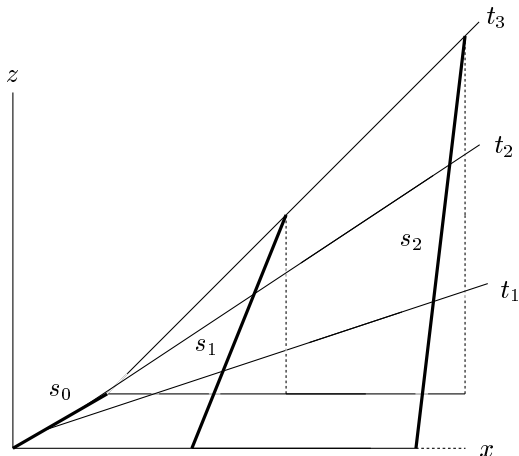
Figure 1: Some of the objects in the construction (for n = 3 ).
