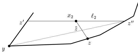
Figure 7: A lower bound for t_2 = \|z - x_2\| .
