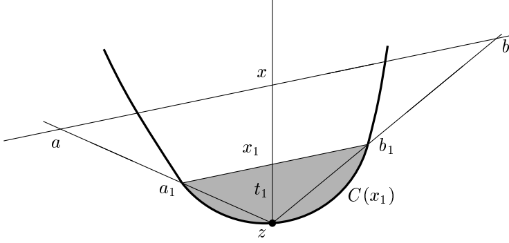
Figure 3: Bounding v(x) .
