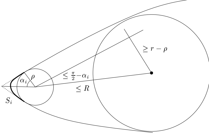
Figure 5: Estimating the length of S .
