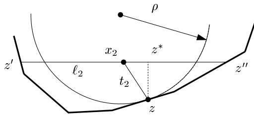
Figure 8: A lower bound on l_2 .
