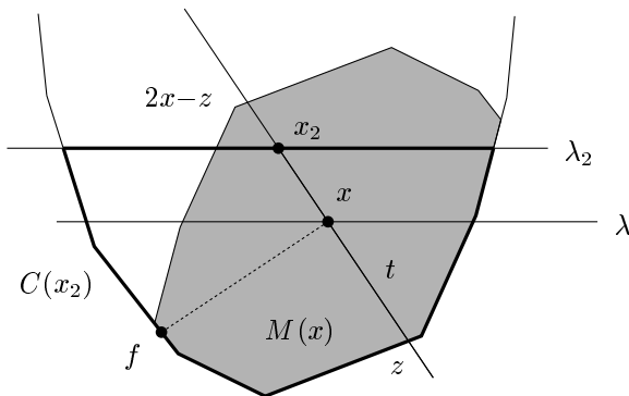
Figure 9: Estimating the width and diameter of M(x) .
