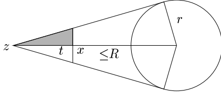
Figure 4: A lower bound for v(x) .
