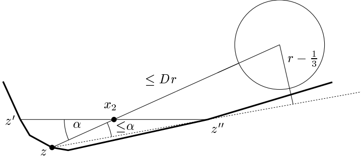
Figure 6: Estimating \alpha .
