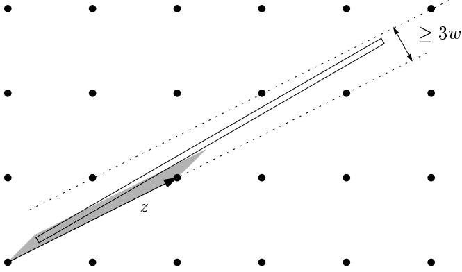
Figure 1: Lattice-point free positions of T
