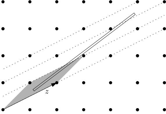
Figure 2: Lattice-point free positions of T ; an upper bound
