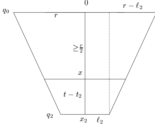
Figure 11: The trapezoid T .
