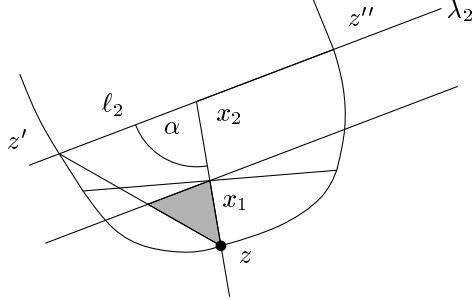
Figure 10: Estimating t_1 .
