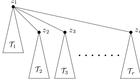
Figure 5: The spider \mathcal{T} constructed in the proof of Lemma 17.
