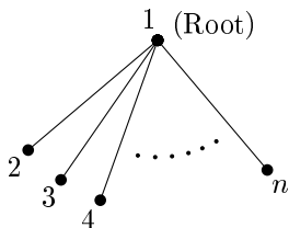
Figure 2: A labeled star giving the lower bound \sigma_u(n) \geq n for any u with |u| > \min\{|u|, 2\} .
