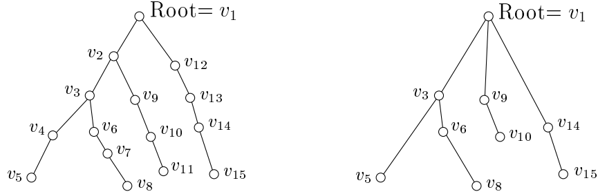
Figure 3: A rooted tree \mathcal{T} and its U -reduction, where U = \{v_1, v_3, v_5, v_6, v_8, v_9, v_{10}, v_{14}, v_{15}\} .
