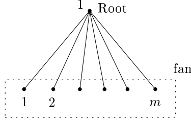
Figure 6: The spider \mathcal{T}(1, m)
