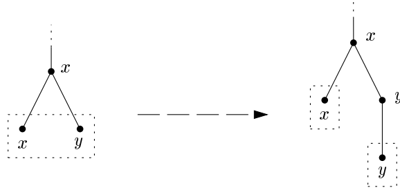
Figure 7: Obtaining \mathcal{T}(k, 1) from \mathcal{T}(k - 1, 2) (dotted rectangles denote fans).
