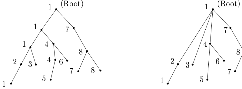
Figure 4: A spider \mathcal{T} and the spider \mathcal{B}(\mathcal{T}, 2) obtained from \mathcal{T} by running the algorithm \mathcal{B}(2) .
