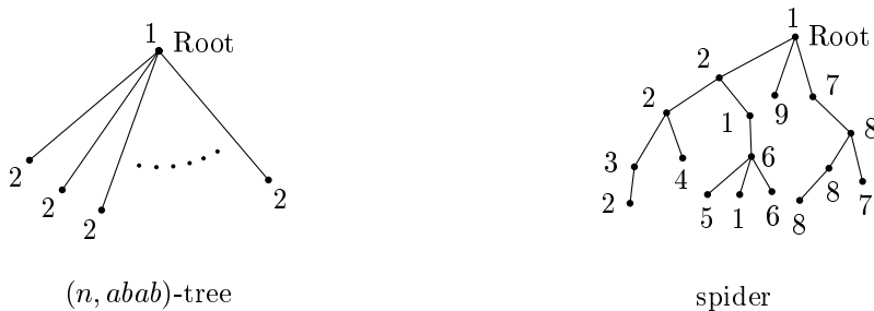
Figure 1: An arbitrarily large (n, abab) -tree (for n \geq 2 ) and an example of a spider.
