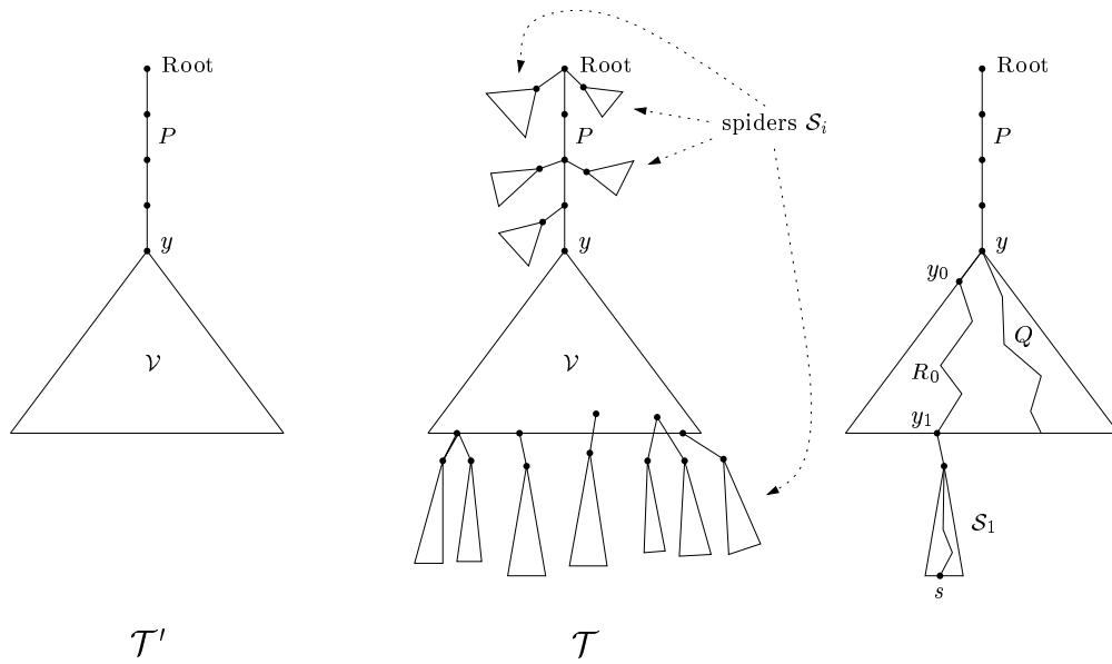
Figure 9: The trees \mathcal{T}' , \mathcal{T} , and the considered paths in \mathcal{T} .
