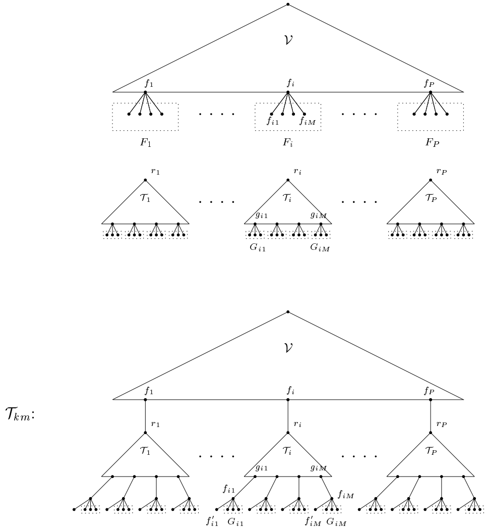
Figure 8: The inductive construction of \mathcal{T}(k, m) , k > 1 , m > 1 .
