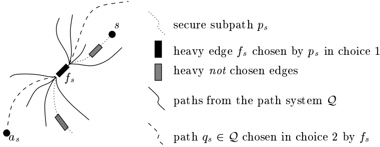
Figure 3: Connection between a secure node s and a node a_s \in W
