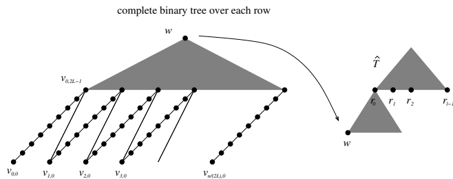
Figure 2: The construction of the network T from a linear array and a binary tree.
