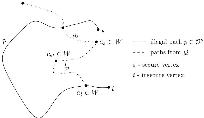
Figure 4: A modification of an illegal path p .
