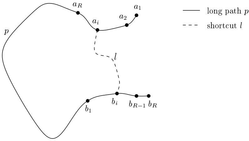
Figure 1: A shortcut l for a long path p \in \mathcal{O}'
