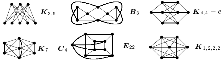
Fig. 2. Examples – 6 of the forbidden minors for the projective plane.
