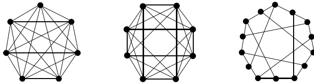
Fig. 3. The graphs K_7 , K_8 - M_4 , and H_{14} .
