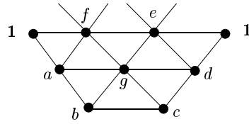
Fig. 4. A straight-ahead walk between two vertices of the same label.
