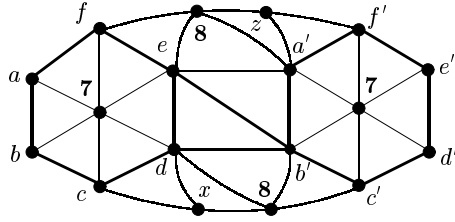
Fig. 6. A fragment of a Klein cover of K_8 - M_4
