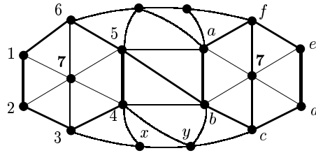
Fig. 5. A fragment of a Klein cover of K_7
