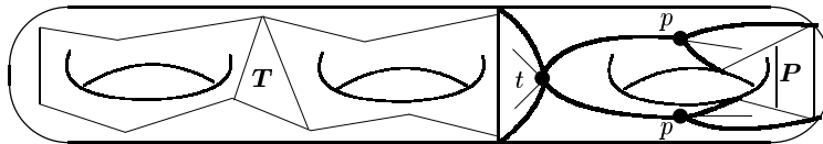
Fig. 7. An emulator of the graph G .
