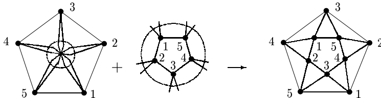
Fig. 1. A double planar cover of K_5 , constructed by lifting its projective drawing
