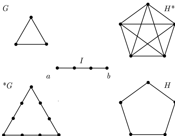
Figure 1: The indicator construction.
