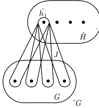
Figure 2: The sub-indicator construction.
