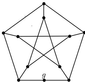
Figure 5: The graph G , \text{girth}(G) = 5 , G \not\rightarrow P_{10} .
