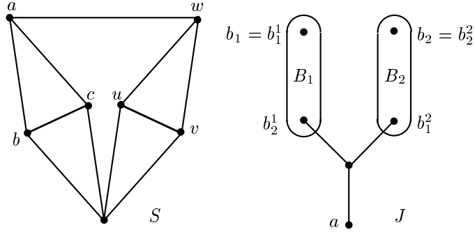
Figure 3: The graph S and the sub-indicator J .
