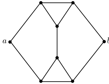
Figure 4: The graph U .
