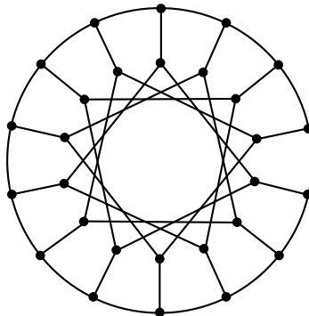
Figure 6: The graph G , \text{girth}(G) = 7 , G \not\rightarrow P_{10} .
