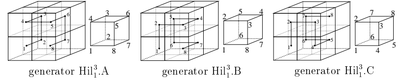
Figure 3: Continuous 3D generators Hil_1^3.x and their canonical corner-indexings Hil_1^3.x .
