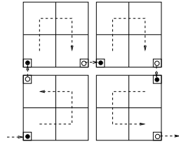
Figure 2: Construction scheme for the 2D Hilbert indexing.
