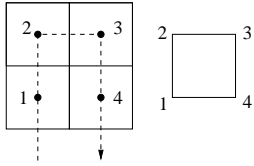
Figure 1: The generator \text{Hil}_1^2 and its canonical corner-indexing \widetilde{\text{Hil}}_1^2 .
