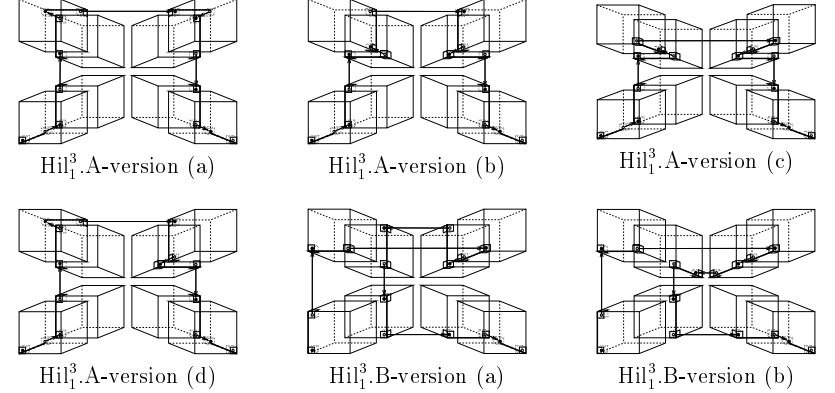
Figure 4: Construction principles for CHPs with generators \text{Hil}_1^3.A and \text{Hil}_1^3.B .
