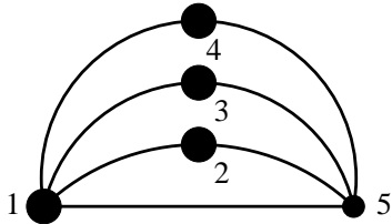
Figure 1: The matroid S_8 is a graft
