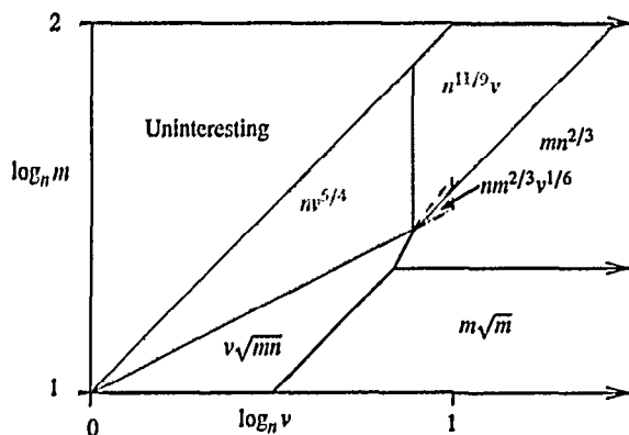
Figure 2: Pictures of the best randomized bounds. (See text for explanation.)
