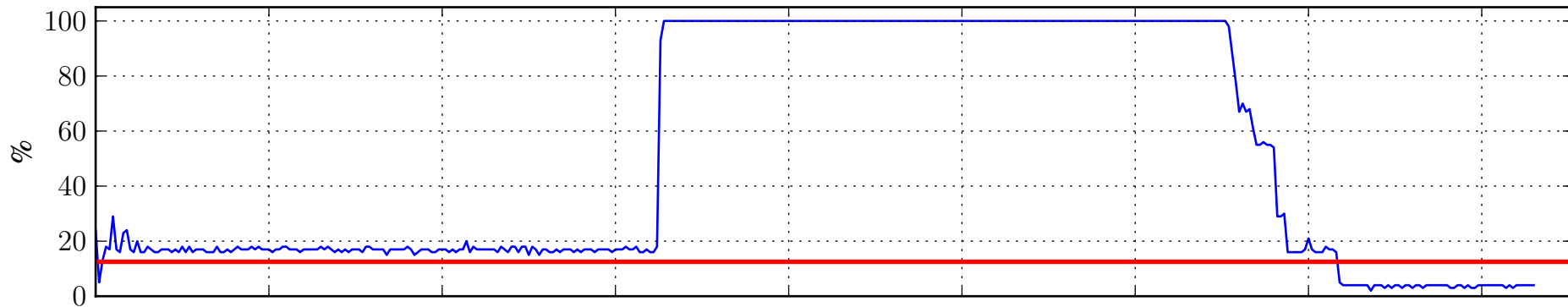
memory usage
