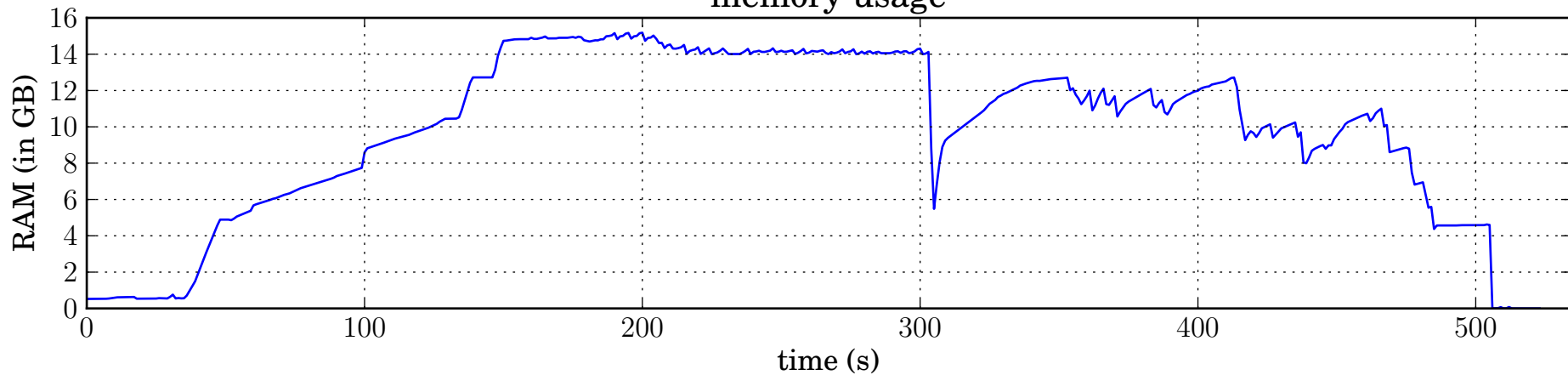
memory usage
