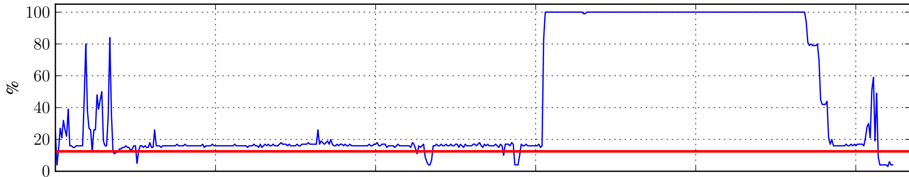
CPU utilization
